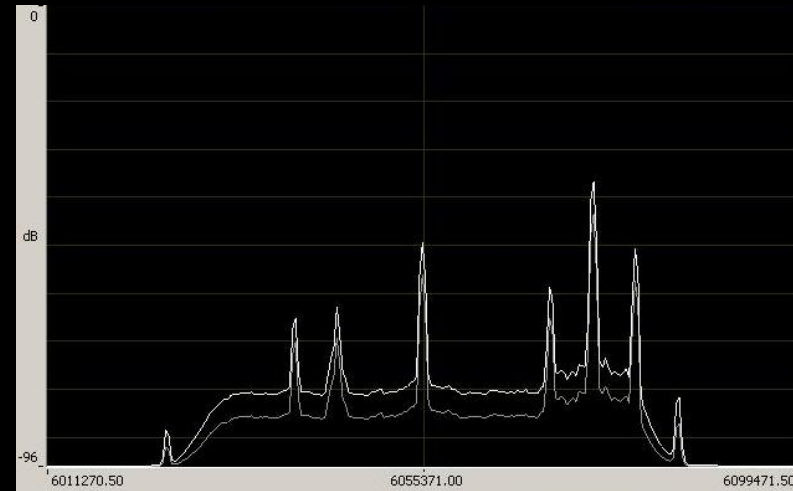
“Entropy”, P , (gray) and Intensity, I , (white) spectra captured by the LOIS receiver in Uppsala 2005-03-15 at 14:25 LT. Peaks are broadcast stations, where P=I . At the noise floor P<I .
