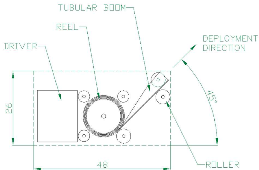
Figure 3: Electric Antenna deployment unit (NanoSpace-1 design by J. Grygorczuk, Space Research Centre, Warsaw, Poland). Scale in mm.
