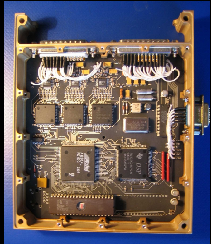
Vector receiver module. Installation on ISS in 2007.
