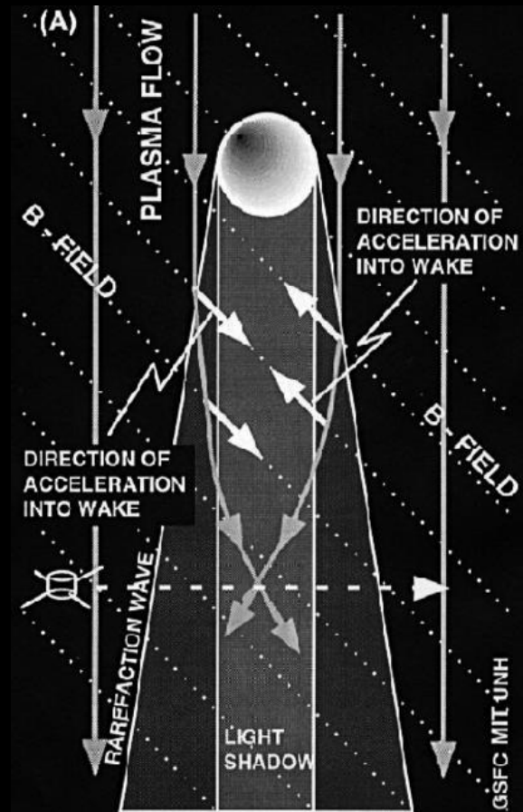
Lunar wake dynamics cartooned from WIND measurements
