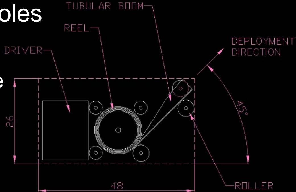
EANT deployment unit, NS1 25 g/1000 mm version.
