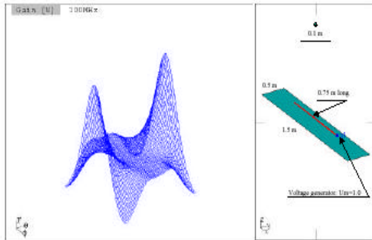
Total radiated far E-field at 100 MHz
