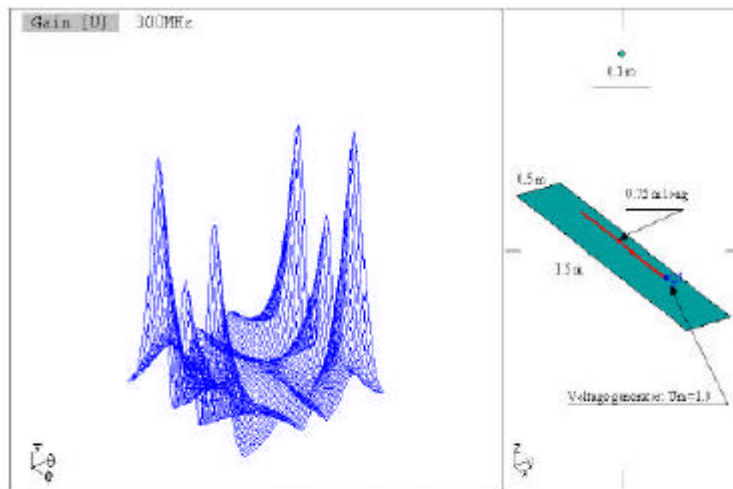
Total radiated far E-field at 300 MHz
